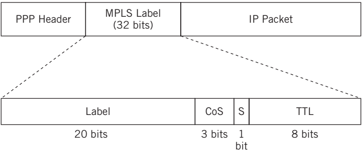
FIGURE 17.6 The 32-bit MPLS label fields. Note the 3-bit CoS field, which is often related to the IP ToS header. The label field is used to identify flows that should be kept together as they cross the network.
