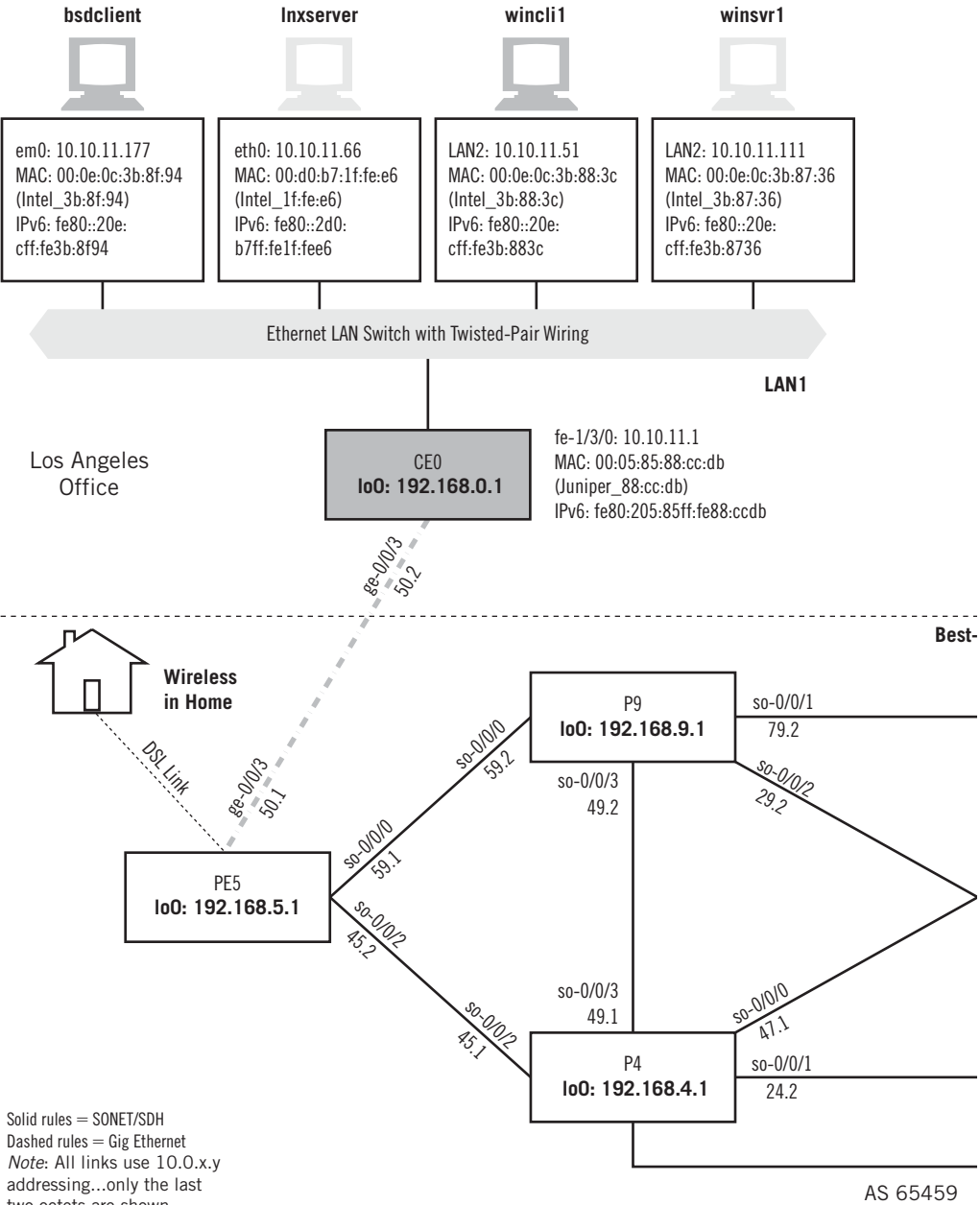
FIGURE 27.1 NAT on the Illustrated Network showing NAT configured on CEO for the use of two hosts on LAN1.
