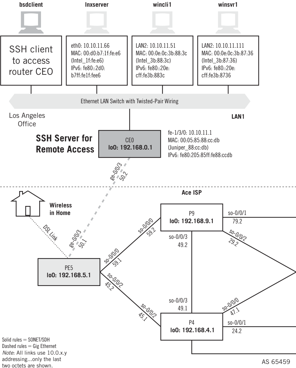
FIGURE 25.1 Using SSH on the Illustrated Network showing the host used as the SSH client and the target router used as the SSH server for remote access.
