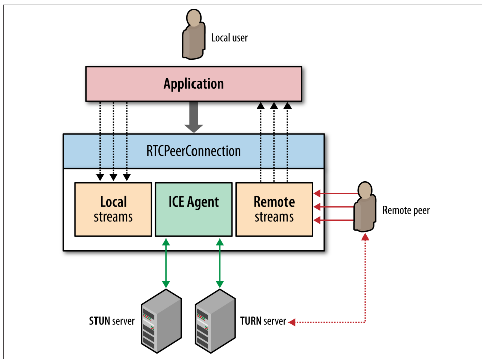
Figure 18-4. RTCPeerConnection API
