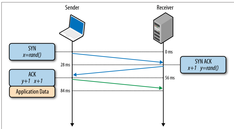
Figure 2-1. Three-way handshake
