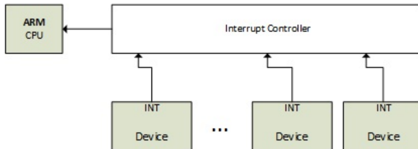
Interrupt controller and IRQ lines
