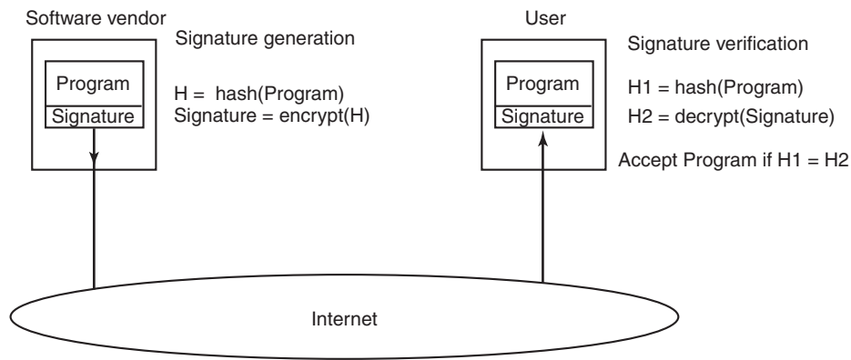
Figure 9-35. How code signing works.
