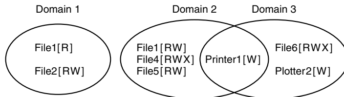
Figure 9-3. Three protection domains.
