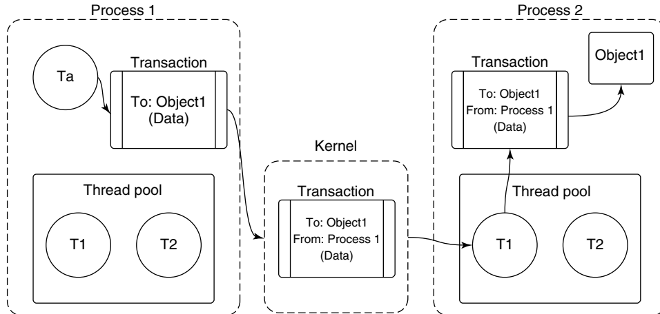
Figure 10-43. Basic Binder IPC transaction.
