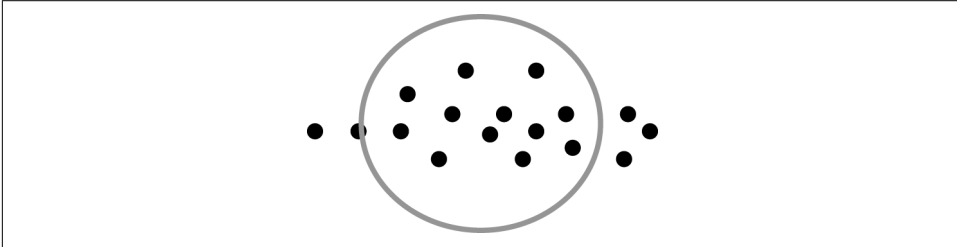
Figure 3-7. Mahalanobis distance
