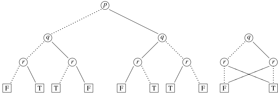
Fig. 5.2 BDD after the Apply and Reduce algorithms terminate
