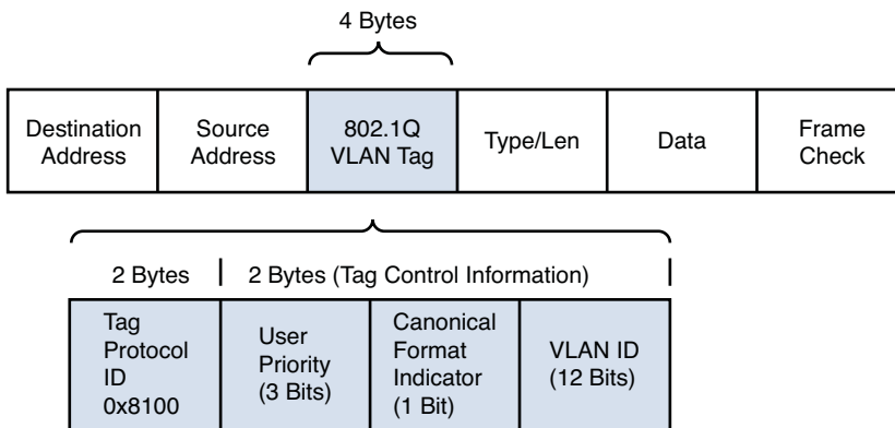
Figure 4.2 An Ethernet frame
