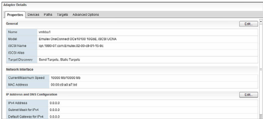
Figure 14.10 Adapter details from an independent hardware iSCSI adapter
