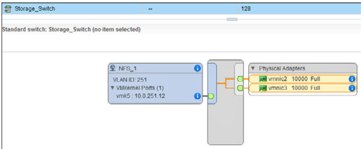
Figure 17.10 The completed and operational Storage_Switch
