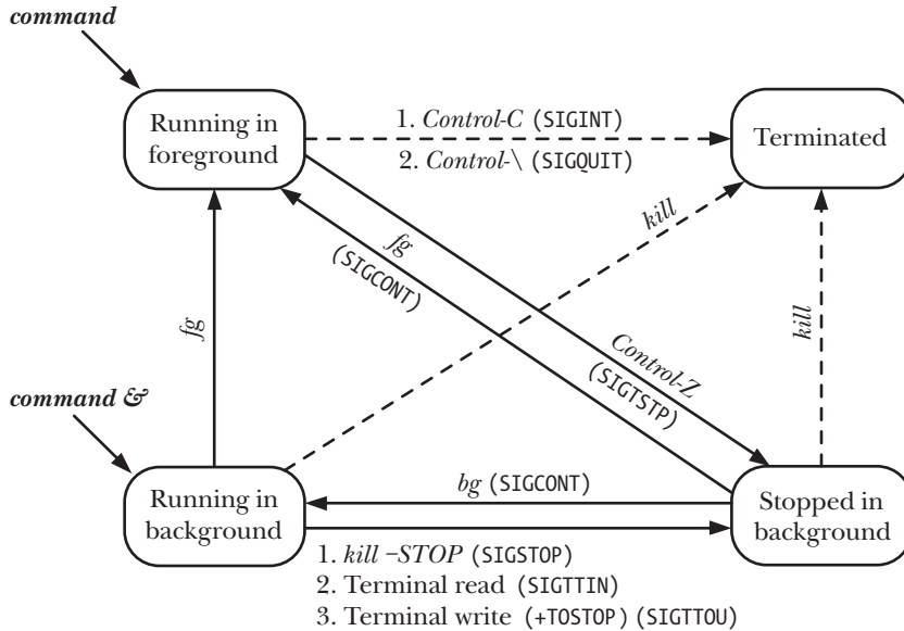
Figure 34-2: Job-control states
