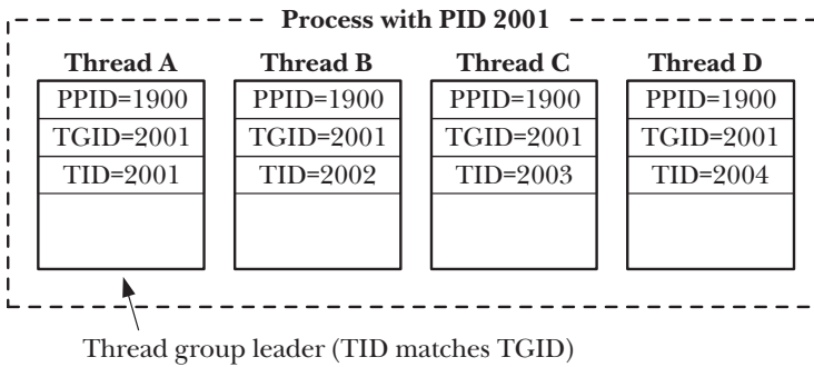
Figure 28-1: A thread group containing four threads
