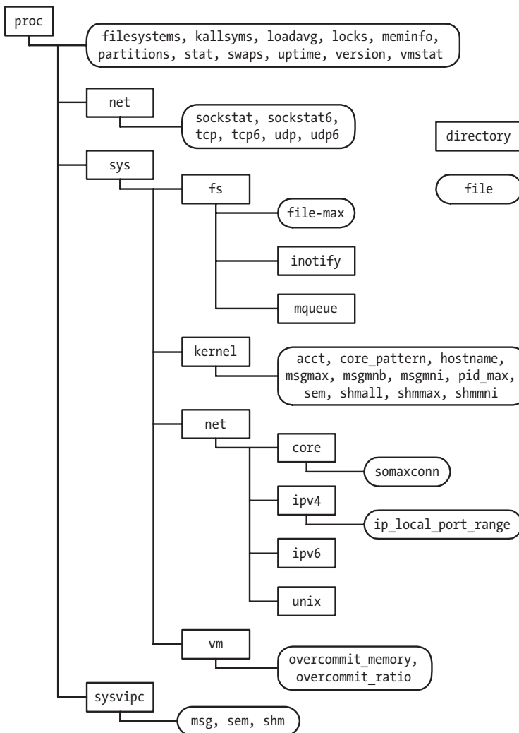
Figure 12-1: Selected files and subdirectories under /proc
