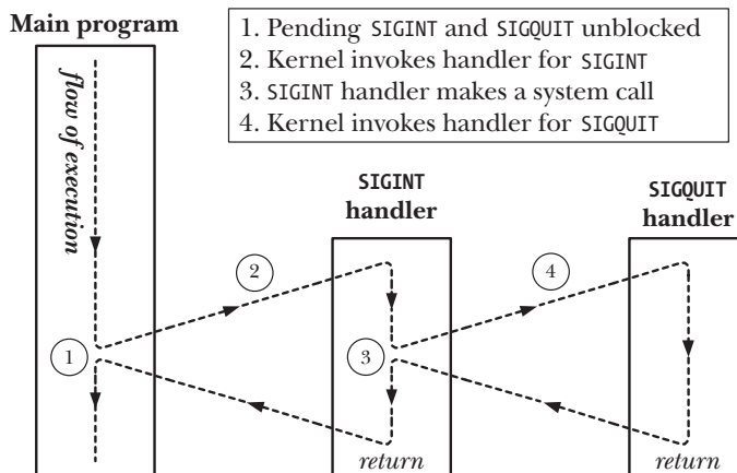
Figure 22-1: Delivery of multiple unblocked signals
