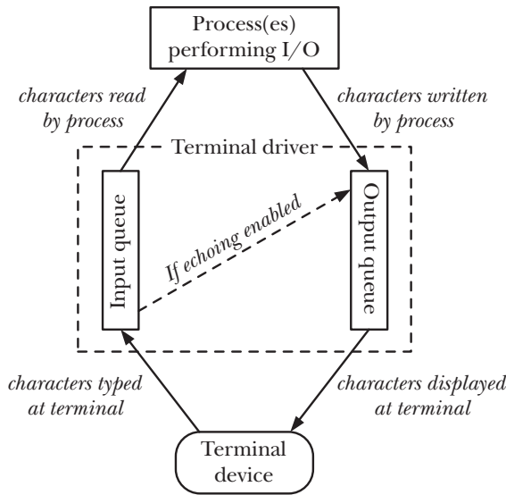
Figure 62-1: Input and output queues for a terminal device
