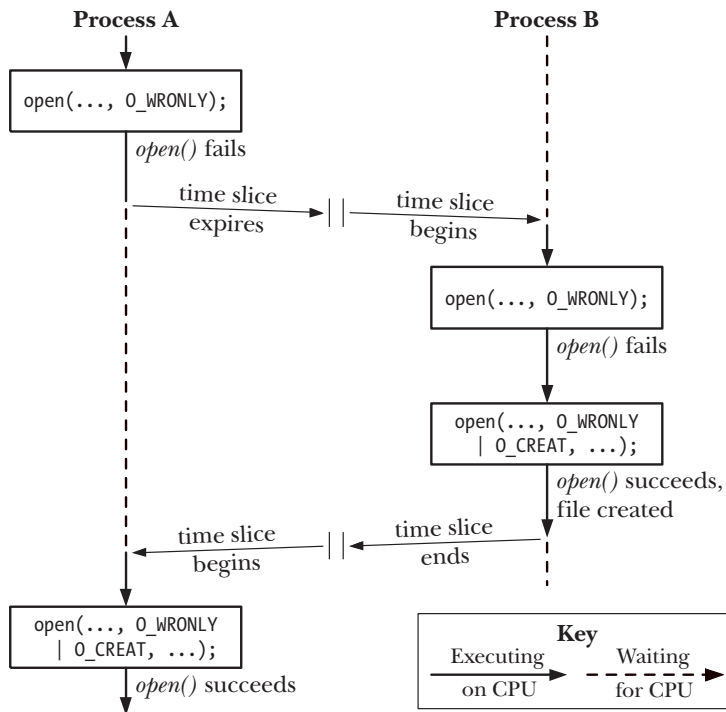
Figure 5-1: Failing to exclusively create a file
