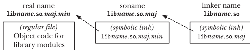
Figure 41-3: Conventional arrangement of shared library names
