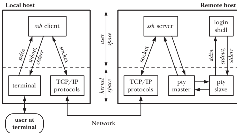
Figure 64-3: How ssh uses a pseudoterminal
