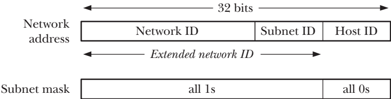
Figure 58-6: IPv4 subnetting
