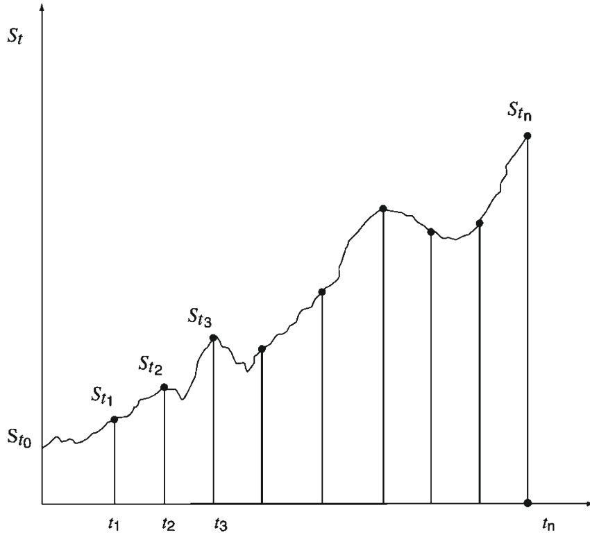
FIGURE 7.1 Discrete time construction of a path based on quantities observed on finite intervals.
