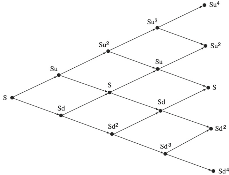
FIGURE 2.1 The multiplicative lattice with up and down movements.
