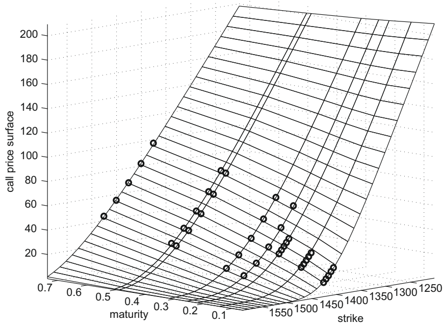
FIGURE 25.4 Call price surface versus market prices.
