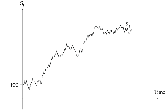
FIGURE 11.2 A sample path of the linear constant coefficient SDE.
