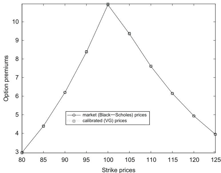
FIGURE 25.5 VG calibrated to Black-Scholes.
