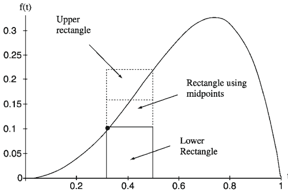
FIGURE 3.10 Illustration of approximating the area under the curve using upper rectangles, lower rectangles, and rectangles using midpoints.
