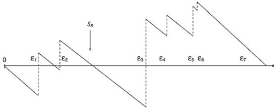
FIGURE 5.8 Construction of a Gaussian process in discrete times.
