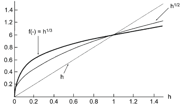
FIGURE 8.3 Plot of h^{r_i} for different choices for r_i .
