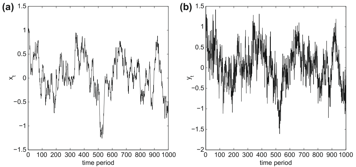
FIGURE 25.9 Filter example: (a) hidden state, (b) observation.
