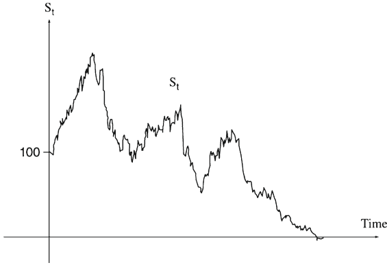
FIGURE 11.5 A sample path of a mean reverting process.
