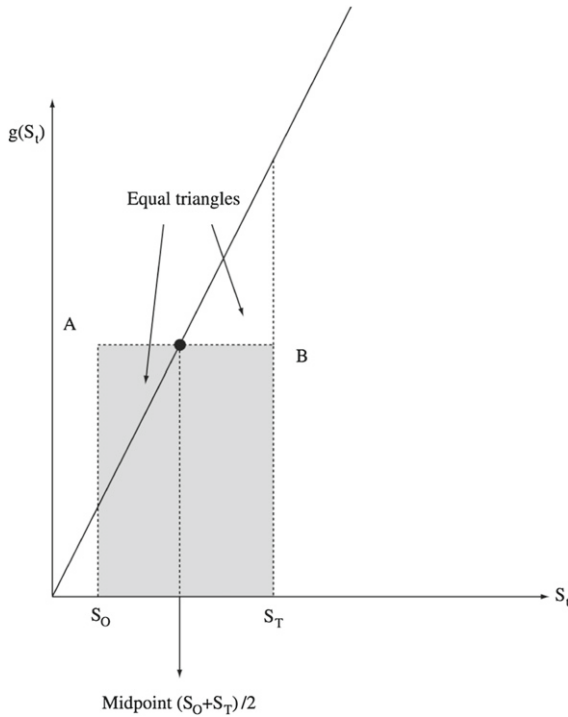
FIGURE 3.11 An example that approximation by rectangles works well.
