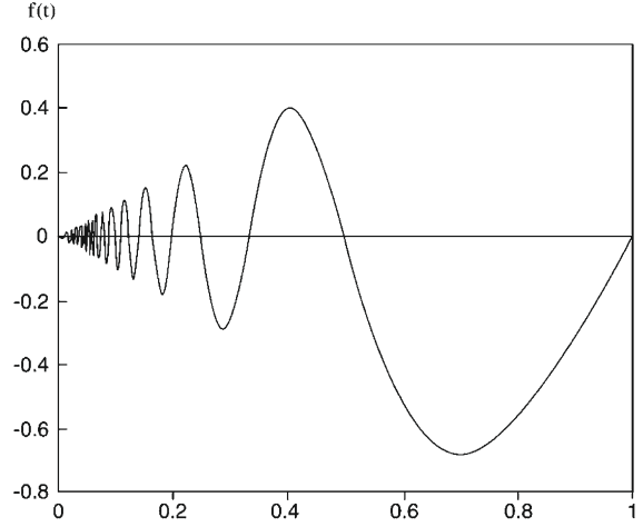
FIGURE 3.2 A plot of a function that is not of bounded variation.
