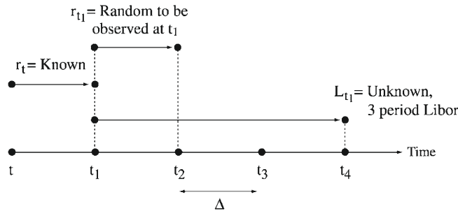
FIGURE 17.2 Effects of the random spot rate r_t
