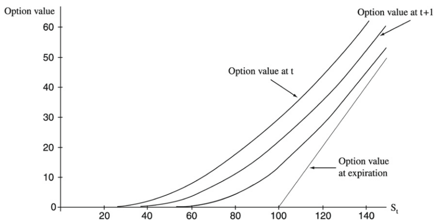
FIGURE 1.4 The value of a call option at various times before its expiration.
