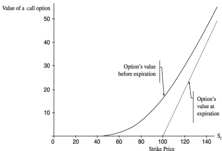
FIGURE 1.3 The relationship between the stock value and the option value before expiration and at expiration.
