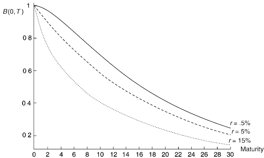
FIGURE 20.1 The graph of the zero-coupon bond at three different levels for the spot rate r = 0.5\% , r = 5\% , r = 15\% .
