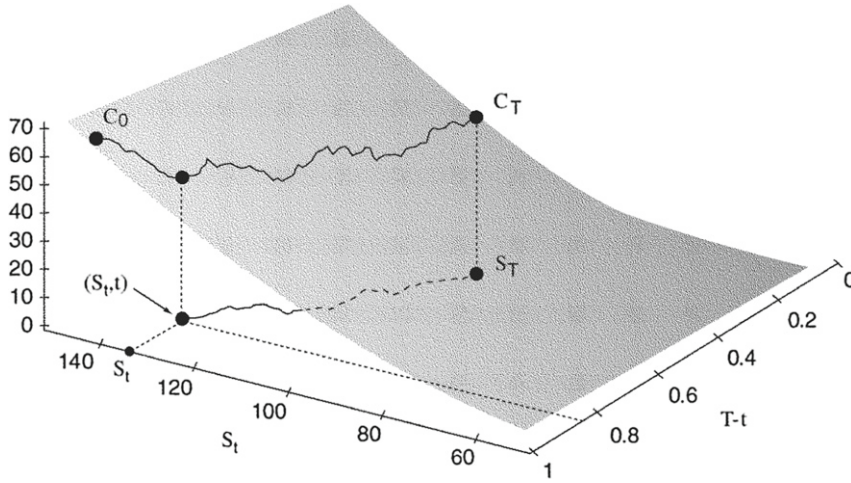
FIGURE 13.6 Random trajectory for the underlying asset price leads to a random path on Black—Scholes surface.
