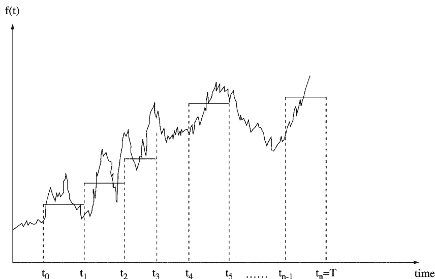
FIGURE 3.9 A example of a function with steep variations that is not Riemann-integrable.
