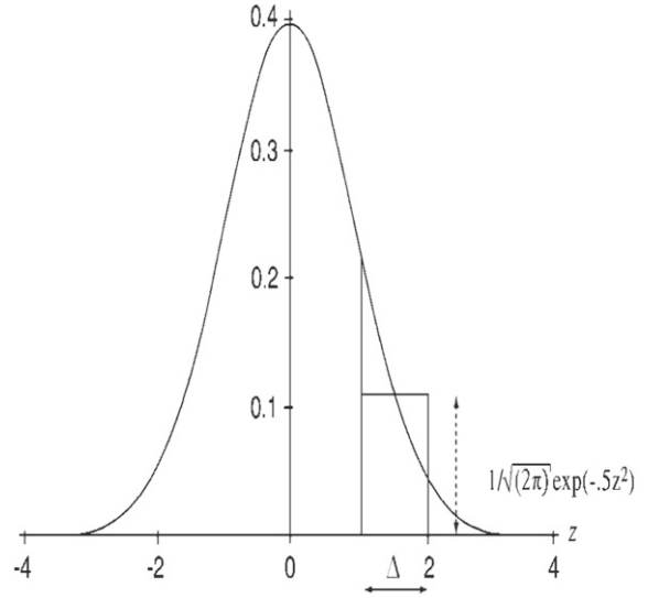
FIGURE 14.1 Calculating the integral of the normal density over a small region using a rectangle.
