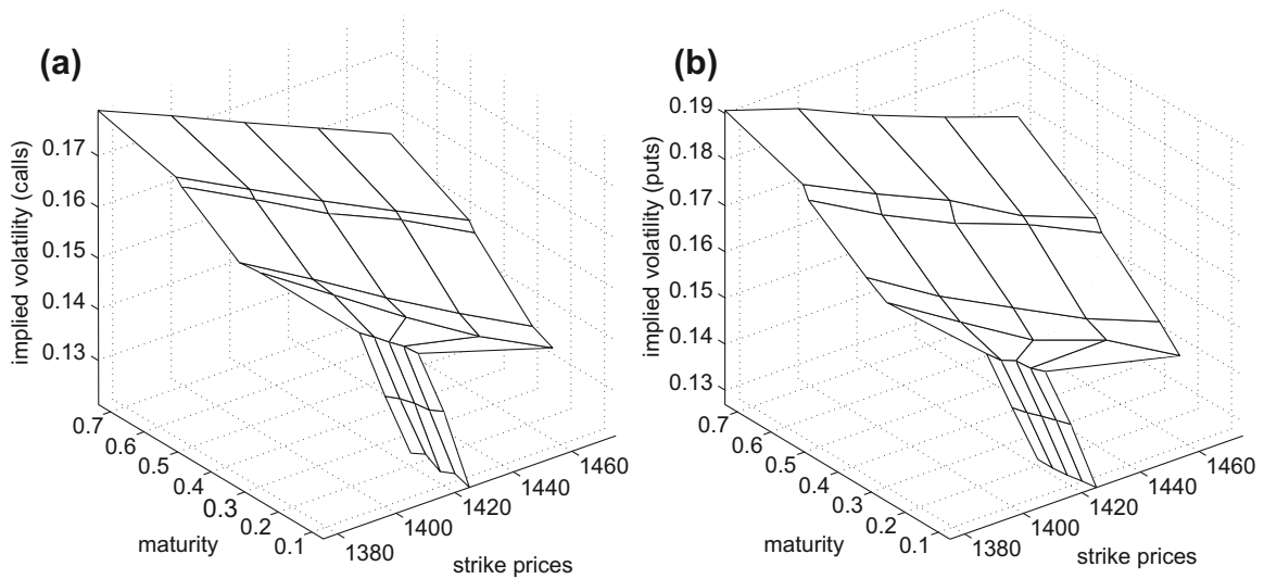
FIGURE 25.1 Implied volatility surface example: (a) calls, (b) puts.
