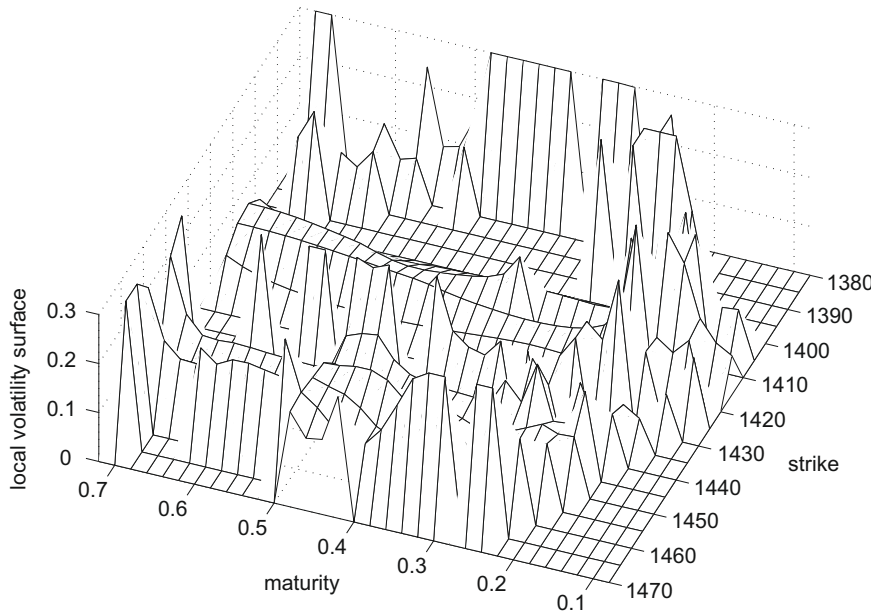
FIGURE 25.2 Local volatility surface obtained from interpolated call prices.
