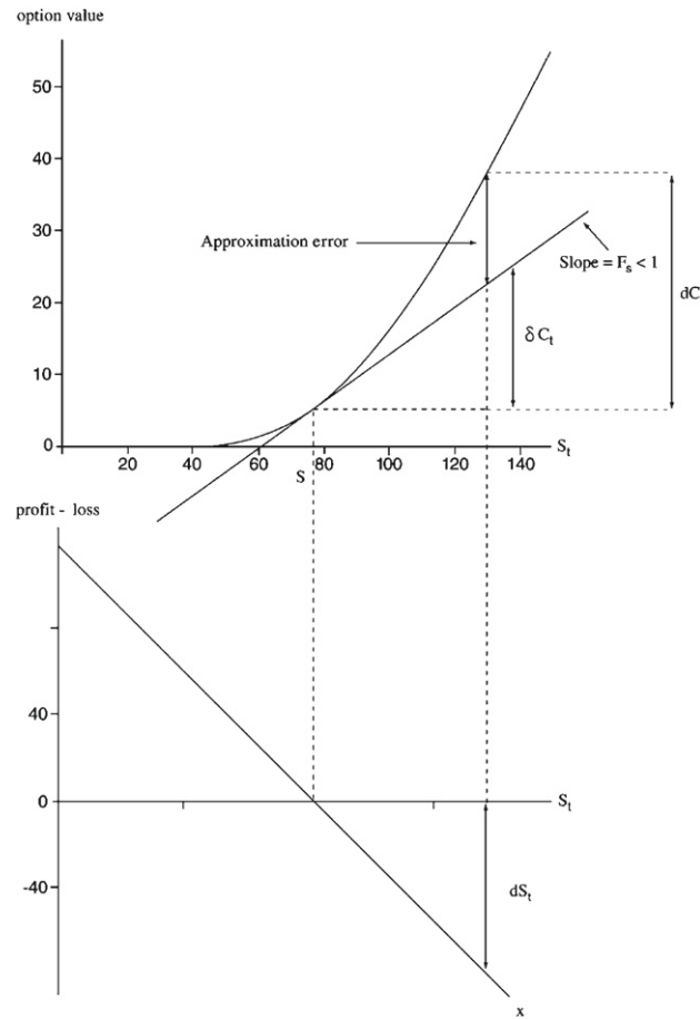
FIGURE 4.2 Change in stock price versus the change in the call option price for the case that the move in stock price is large.
