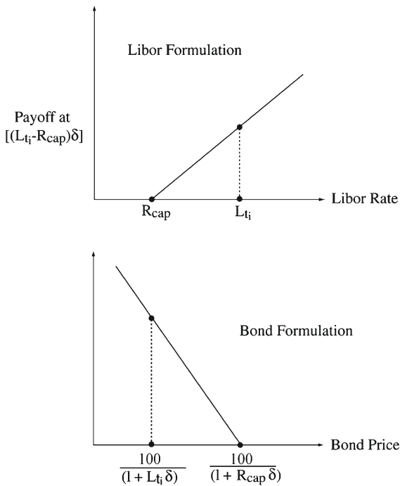
FIGURE 16.2 Interest rate caps.
