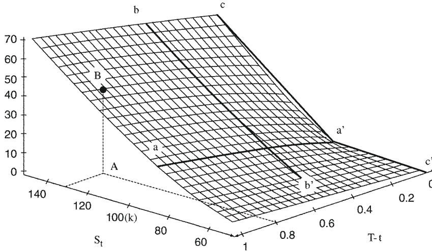
FIGURE 13.1 Black-Scholes call price surface.
