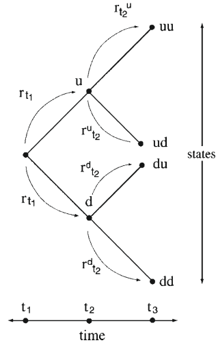
FIGURE 17.1 Illustration of randomness of risk-free rate.
