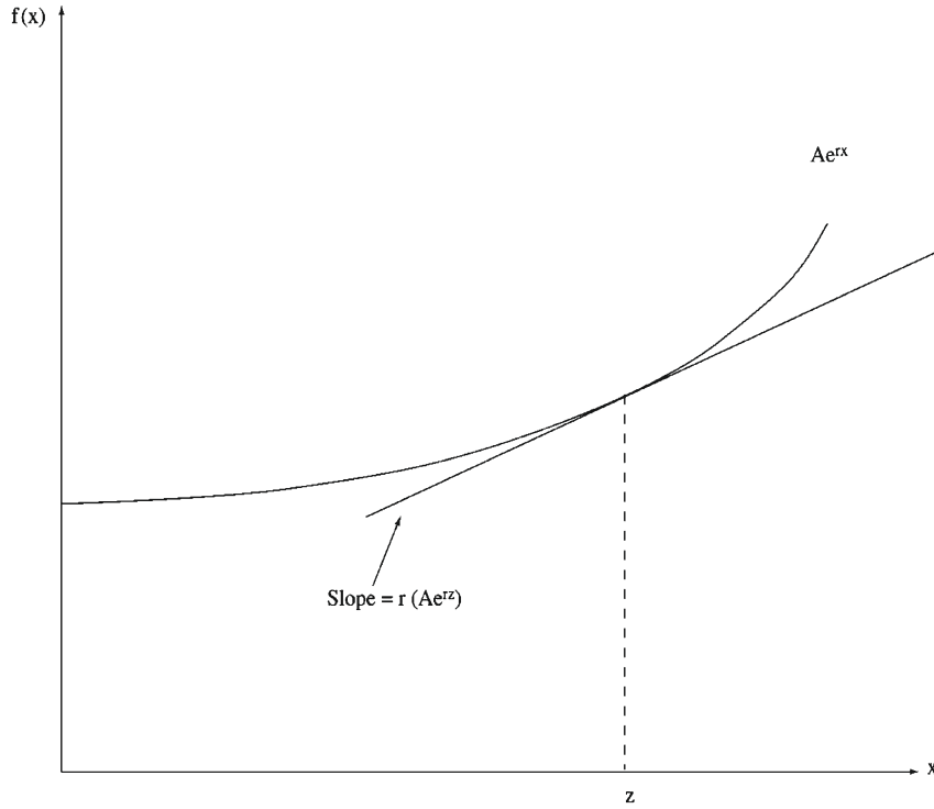
FIGURE 3.3 Graphical illustration of the slope of an exponential function.
