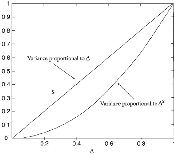
FIGURE 5.4 Difference between a variance proportional to \Delta and one proportional to \Delta^2 .
