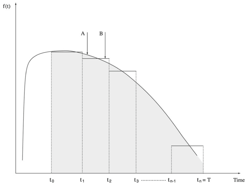
FIGURE 3.8 The construction steps to find the area under the graph via the Riemann integral.
