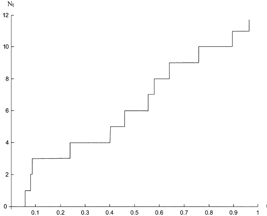
FIGURE 8.1 A Poisson process sample path.
