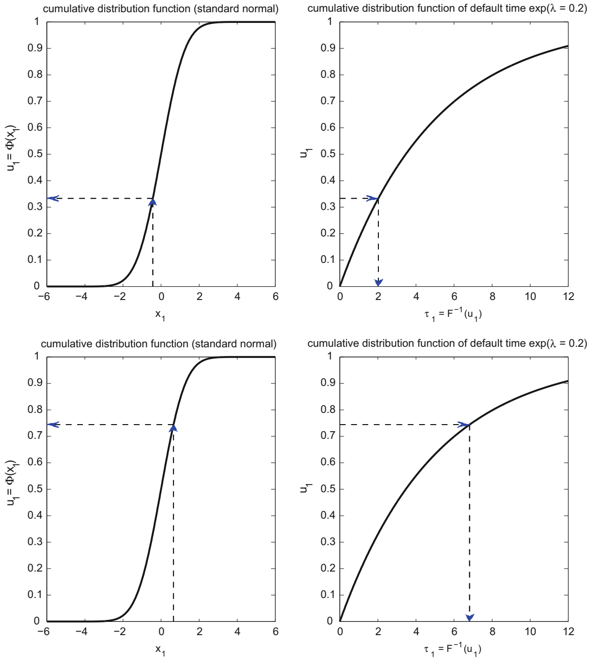
FIGURE 23.3 Mapping a standard normal random variable to a default time.
