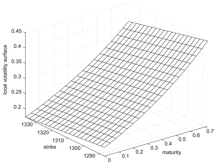
FIGURE 25.3 Local volatility surface obtained using a functional form for the local volatility surface.
