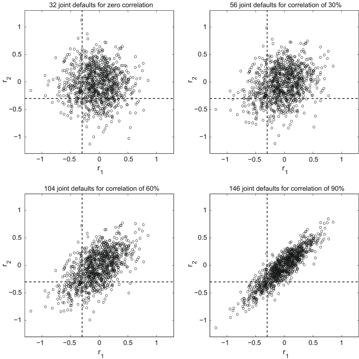
FIGURE 23.2 Default correlation for various correlation scenarios for two obligors.
