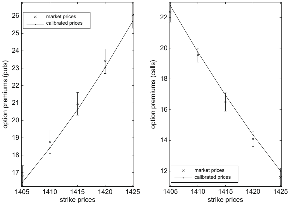
FIGURE 25.6 Variance gamma versus market premiums for the S&P 500 on March 27, 2012 for time to maturity of 24 days.
