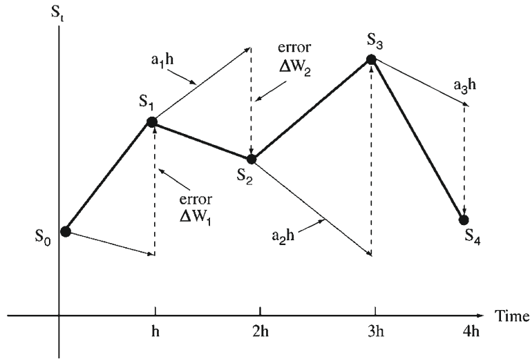
FIGURE 11.1 A sample path of a geometric SDE on discrete intervals of length h .
