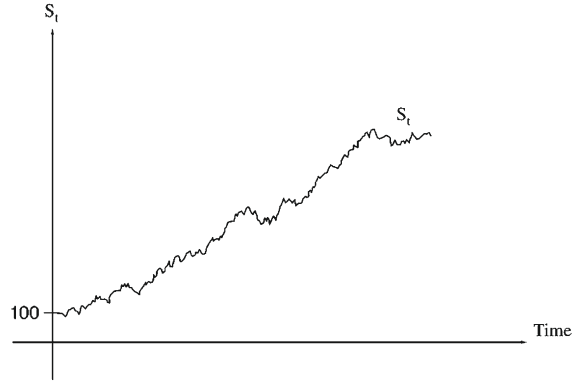
FIGURE 11.4 A sample path of square root process.
