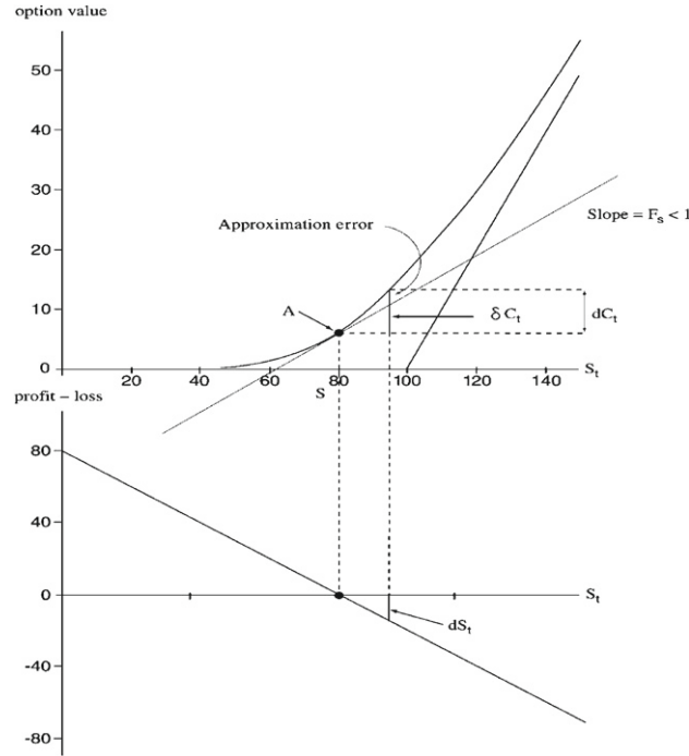
FIGURE 4.1 Change in stock price versus the change in the call option price.
